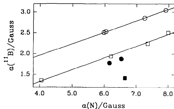
Fig. 7. Dependence of the ^{11}\text{B} hyperfine splitting on a(\text{N}) in the \text{BH}_3 ( \circ ) and \text{BPh}_3 ( \square ) complexed radical anions of N -heterocycles. Radicals derived from species 9 and 10 are indicated by the filled symbol.
