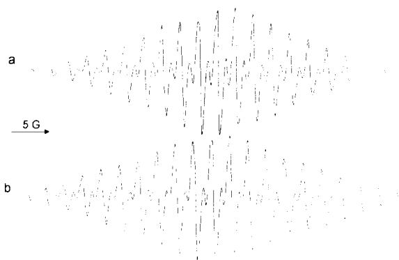
Fig. 2. Experimental (a) and simulated (b) EPR spectrum of radical 1f recorded in THF at room temperature. Spectrum (b) has been simulated taking into account the presence of the isotopomeric species containing ^{10}\text{B} and ^{11}\text{B} .
