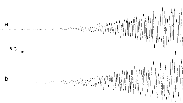
Fig. 3. Experimental (a) and simulated (b) half EPR spectrum of radical 2d , recorded in benzene at room temperature.
