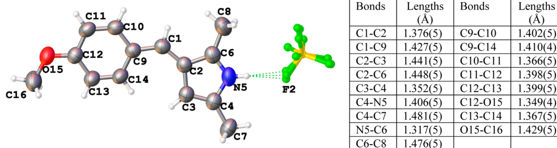
Figure 1. Asymmetric unit of compound 3i with atom labeling (displacement ellipsoids for all but hydrogen and fluorine atoms are drawn at 50% probability) and relevant cation bond distances.
