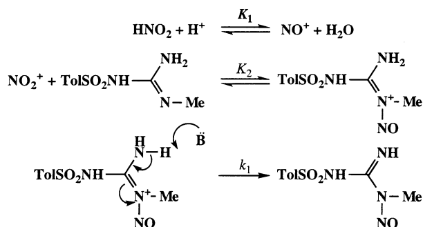
Scheme 1 Mechanism of the nitrosation of TSG
