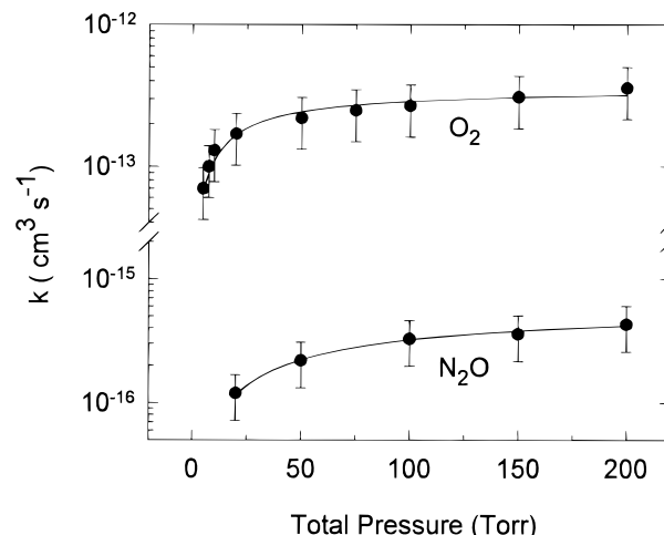
Figure 6. Pressure dependence of the reaction of \text{Ir}(a^4F_{9/2}) with O 2 and N 2 O in N 2 buffer at room temperature. Error bars represent \pm 40\% uncertainty. The solid lines are fits to eq 3.
