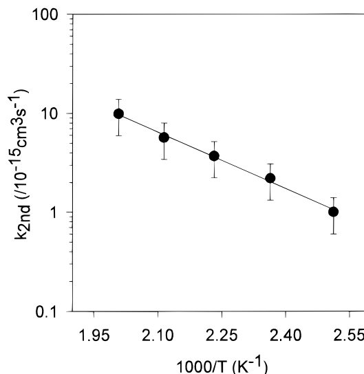
Figure 5. Arrhenius plot for the collisional disappearance of \text{Ir}(a^4F_{9/2}) with CH 4 . Error bars represent \pm 40\% uncertainty.
