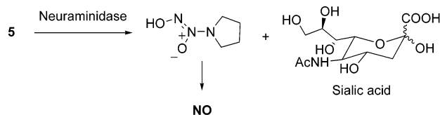
Scheme 2. NO-Releasing Mechanism of 5
