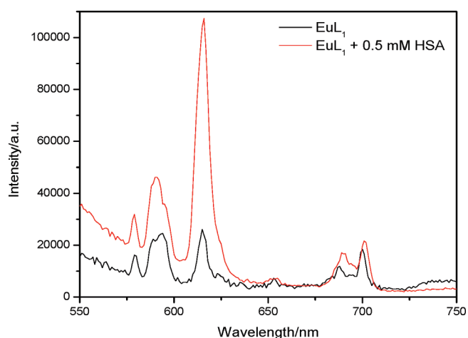
Figure 4. Responsive europium emission enhanced and ratio changes after 10 \mu\text{M} \text{EuL}_2 bound with 0.5 mM HSA in HEPES.
