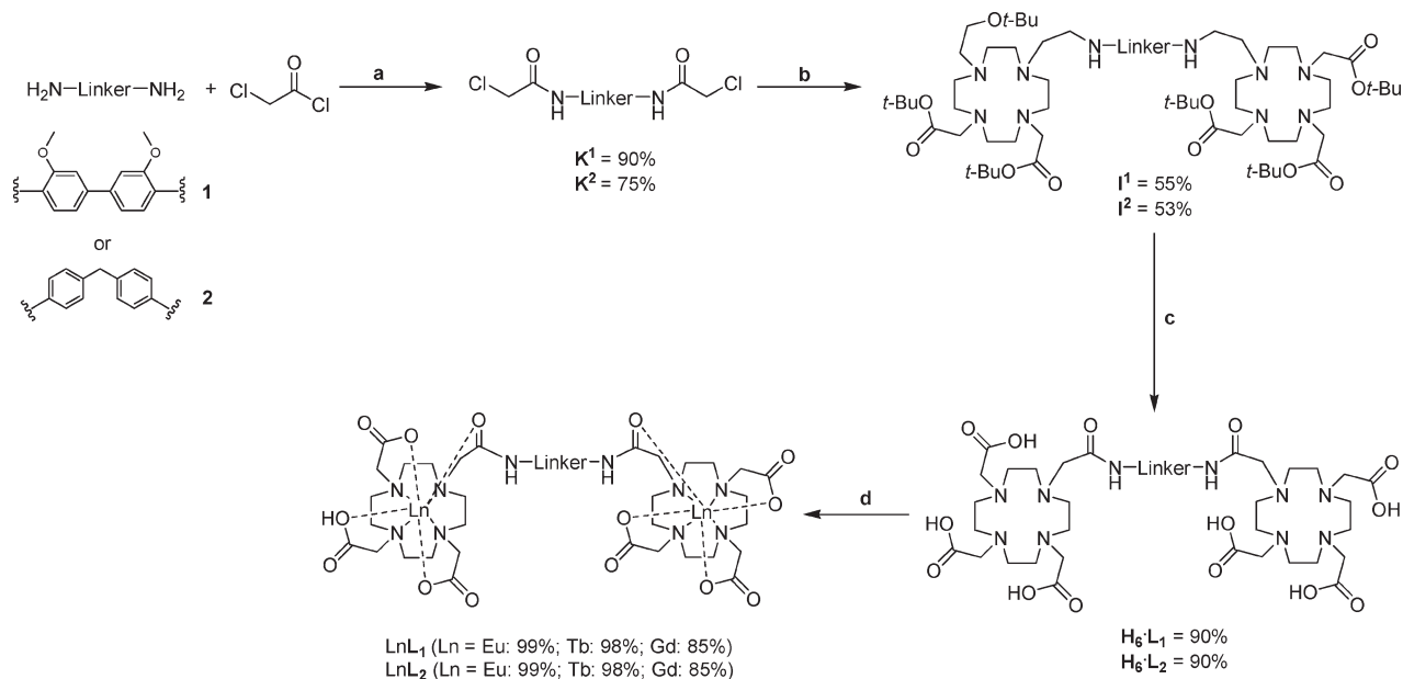
Scheme 1. Reaction Schemes of Dimeric Lanthanide Complexes ( \text{LnL}_1\text{--LnL}_2 , \text{Ln} = \text{Eu, Tb, and Gd} ) a
