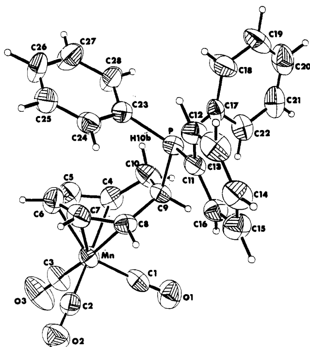
Figure 1. Structure and atom numbering scheme for the cation in [(\text{PPh}_3\text{C}_7\text{H}_8)\text{Mn}(\text{CO})_3]\text{BF}_4 .
