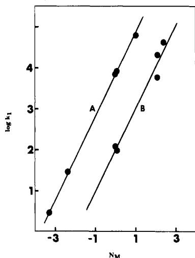
Figure 2. Plot of reactivity vs. N_M according to eq 4: (A) (\text{C}_7\text{H}_8)\text{Mn}(\text{CO})_3^+ ; (B) (\text{C}_7\text{H}_8)\text{Mn}(\text{CO})_2\text{L}^+ .
