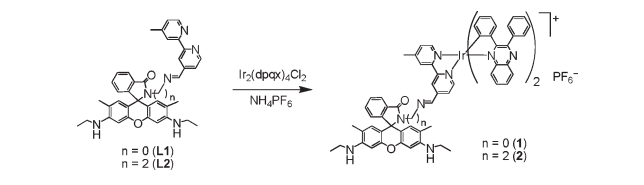
Scheme 1. Synthetic Route of 1 and 2
