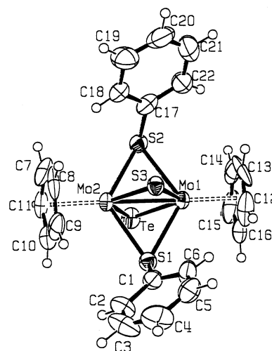
Fig. 1. Molecular structure of \text{Cp}_2\text{Mo}_2(\mu\text{-S})(\mu\text{-Te})(\mu\text{-SPh})_2 ( 1 ).
