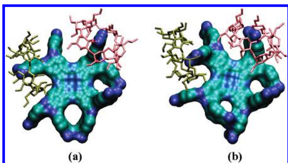
Figure 4. The initial (a) and final (b) configurations of 3-(\beta\text{-CD})_2 (two \beta\text{-CD} rings trapping two intervening carboxyphenoxy groups), revealing the incipient departure of the \beta\text{-CD} rings in explicit water solvent molecules (being omitted for clarity) after 2 ns MD simulation with use of AMBER 8.0. The phthalocyanine and the \beta\text{-CD} molecules are rendered as a molecular surface and stick representation, respectively.
