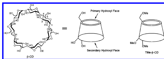
Figure 1. Schematic structures of \beta -CD and TMe- \beta -CD.
