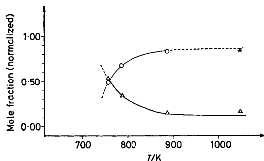
FIGURE 4 Molar fractions (normalized) of oxathiiran (10) ( \Delta ) and thioketen (9) ( \circ ) as a function of thermolysis temperature. The point X corresponds to the theoretical amount of thioketen taking the amount of carbene (5) into account
