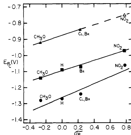
Figure 2. Correlation of E_p (V) with the Hammett \sigma_p parameter for the molybdenum(VI) complexes: \bullet , \text{MoO}_2(5\text{-X-SAE}) ; \blacksquare , \text{MoO}_2(5\text{-X-SAP}) ; \blacktriangle , \text{MoO}_2(5\text{-X-SAN}) ; \Delta , predicted ( X = \text{CH}_3\text{O} , \text{H} , \text{Cl} , \text{Br} , \text{NO}_2 ).
