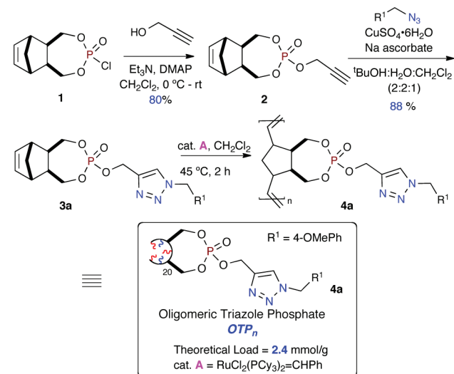
Scheme 1. Synthesis of Oligomeric Triazole Phosphate (OTP) 4a
