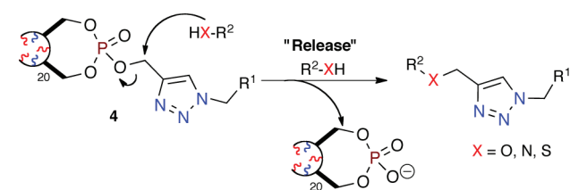
Figure 1. Reaction of oligomeric triazole phosphate (OTP) 4 .
