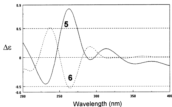
Figure 3. CD spectra of compounds 5 and 6.
