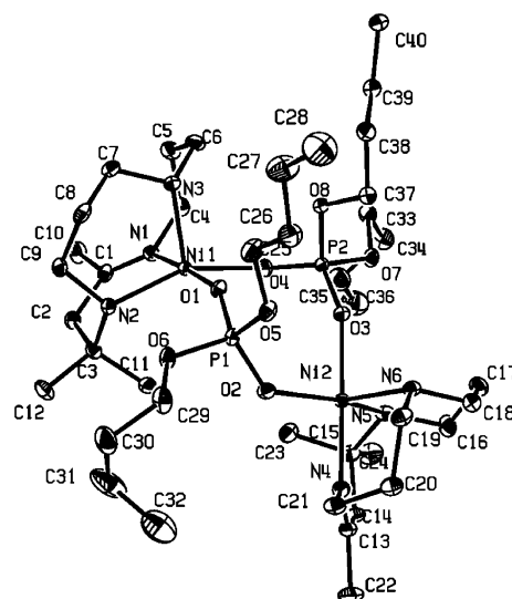
Figure 3. ORTEP plot of the cation of [[\text{Ni}(\text{Me}_3[12]\text{aneN}_3)(\mu\text{-O}_2\text{P}(\text{OBu})_2)_2](\text{PF}_6)_2] ( 2 ).
