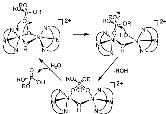
Scheme 3. Proposed molecular mechanism for the hydrolysis of phosphate triesters in the presence of a dinuclear Ni II complex.
