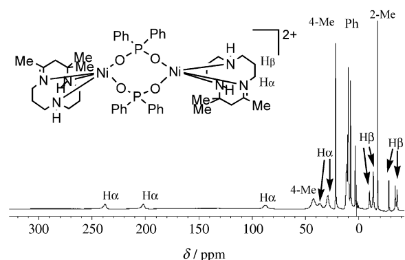
Figure 2. ^1\text{H} NMR spectra (in [\text{D}_6]\text{acetone} at room temperature) of compound 10 .
