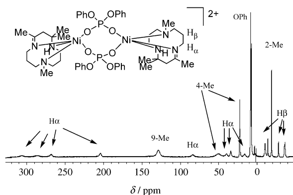
Figure 1. ^1\text{H} NMR spectra (in [\text{D}_6]\text{acetone} at room temperature) of compound 7 .
