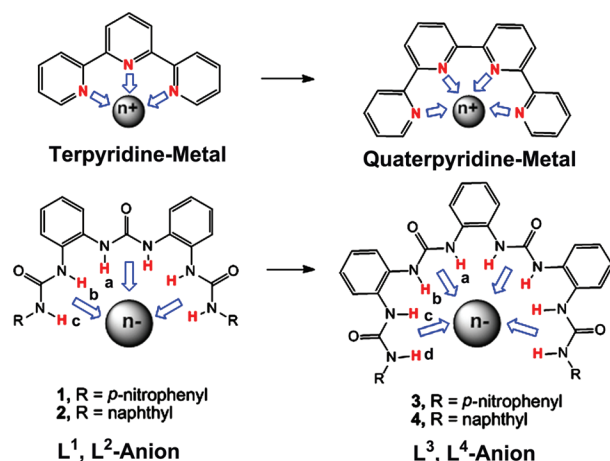
Scheme 1. The Design Strategy of Triurea and Tetraurea Based Anion Receptors
