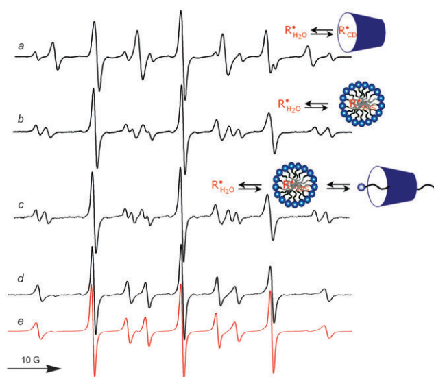
Fig. 1 EPR spectra of TBBN recorded in water at 298 K. (a) DM-β-CD 5.3 mM; (b) SDS 33 mM; (c) β-CD 16 mM and SDS 49 mM; (d) DM-β-CD 16 mM and SDS 49 mM. (e) Theoretical simulation of spectrum (d) obtained with the rate constant reported in Table 1, entry 11.
