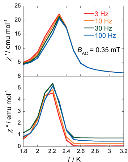
Figure 4. The temperature dependencies of \chi' and \chi'' of 1 measured under DC and AC fields of B_{\text{DC}} = 0 and B_{\text{AC}} = 0.35 mT.
