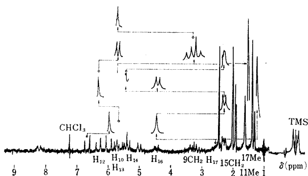
Fig. 3. NMR Spectrum of 8-Oxo Lankacidin A (XV) 100 MHz, CDCl 3
