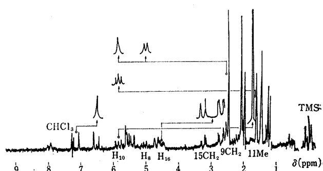
Fig. 4. NMR Spectrum of 14-Oxo-lankacidin C, 8-Acetate (XVI) 100MHz, CDCl 3
