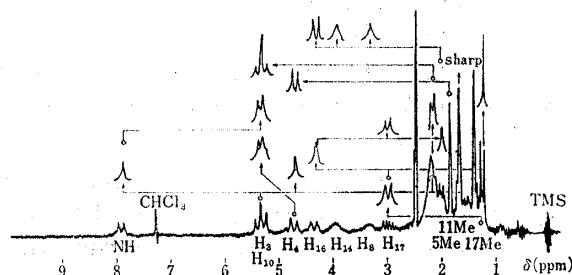
Fig. 2. NMR Spectrum of 6,7,12,13-Tetrahydro Lankacidin C (X) 100 MHz, \text{CDCl}_3
