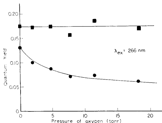
Figure 6. Quenching of the formation of products by oxygen: ■, cis -1-phenyl-2-butene; ●, 1-phenyl-2-methycyclopropane; pressure of trans -1-phenyl-2-butene, 0.8 Torr; temperature, 26°.
