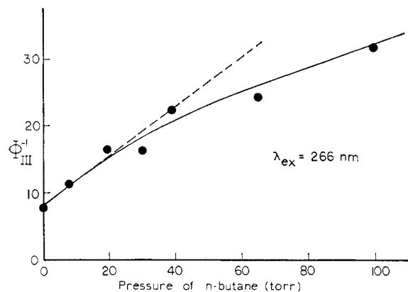
Figure 8. Reciprocal of the quantum yield of formation of 1-phenyl-2-methylcyclopropane vs. n -butane pressure: pressure of I, 0.8 Torr; temperature, 26°.
