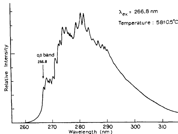
Figure 3. Fluorescent spectrum of trans -1-phenyl-2-butene: spectral resolution, 0.24 nm.
