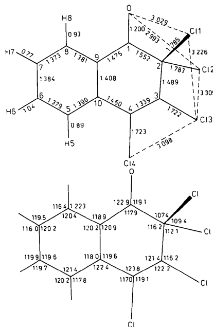
Fig. 3. Bond lengths (Å) and valence angles (°) of the \alpha -TKN molecule.
