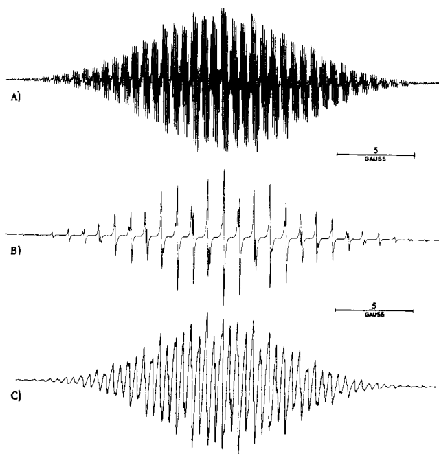
Figure 2. Computer-simulated ESR spectra of the radical anions of [2.2]paracyclophane (A and B) and its 4,12-dideuterio derivative (C). Coupling parameters used (in gauss): (A) a_H' = 3.78 , a_H'' = 1.96 , a_H''' = 1.27 , and a_H'''' = 0.68 , each for four equivalent protons, and a_K = 0.120 for one ^{39}\text{K} nucleus; (B) \bar{a}_H' = 2.97 and \bar{a}_H'' = 1.03 , each for eight equivalent protons; (C) 86%, \bar{a}_H' = 2.97 and \bar{a}_H'' = 1.03 , for six and eight equivalent protons, respectively, and a_D = 0.46 for two equivalent deuterons; 14%, \bar{a}_H' = 2.97 and \bar{a}_H'' = 1.03 , for seven and eight equivalent protons, respectively, and a_D = 0.46 for one deuteron.
