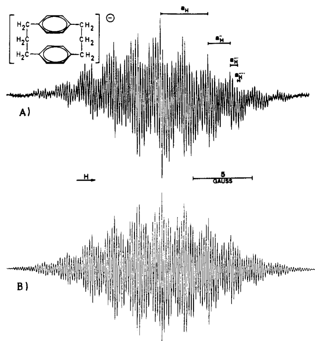
Figure 3. ESR spectra of the radical anion of [3.3]paracyclophane: (A) solvent 1,2-dimethoxyethane with 2–3% hexamethylphosphoramide, temperature -90^{\circ} ; (B) computer-simulated spectrum. Coupling parameters used (in gauss): a_H' = 3.95 , a_H'' = 1.88 , a_H''' = 0.575 , and a_H'''' = 0.192 , each for four equivalent protons.
