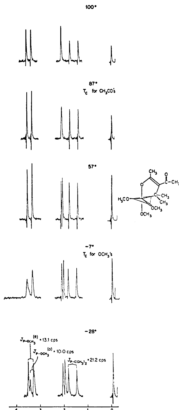
Figure 1. Temperature dependence of the nmr spectrum of the adduct 3 of trimethyl phosphite and isopropylideneacetylacetone (60 Mc; bromobenzene as solvent).
