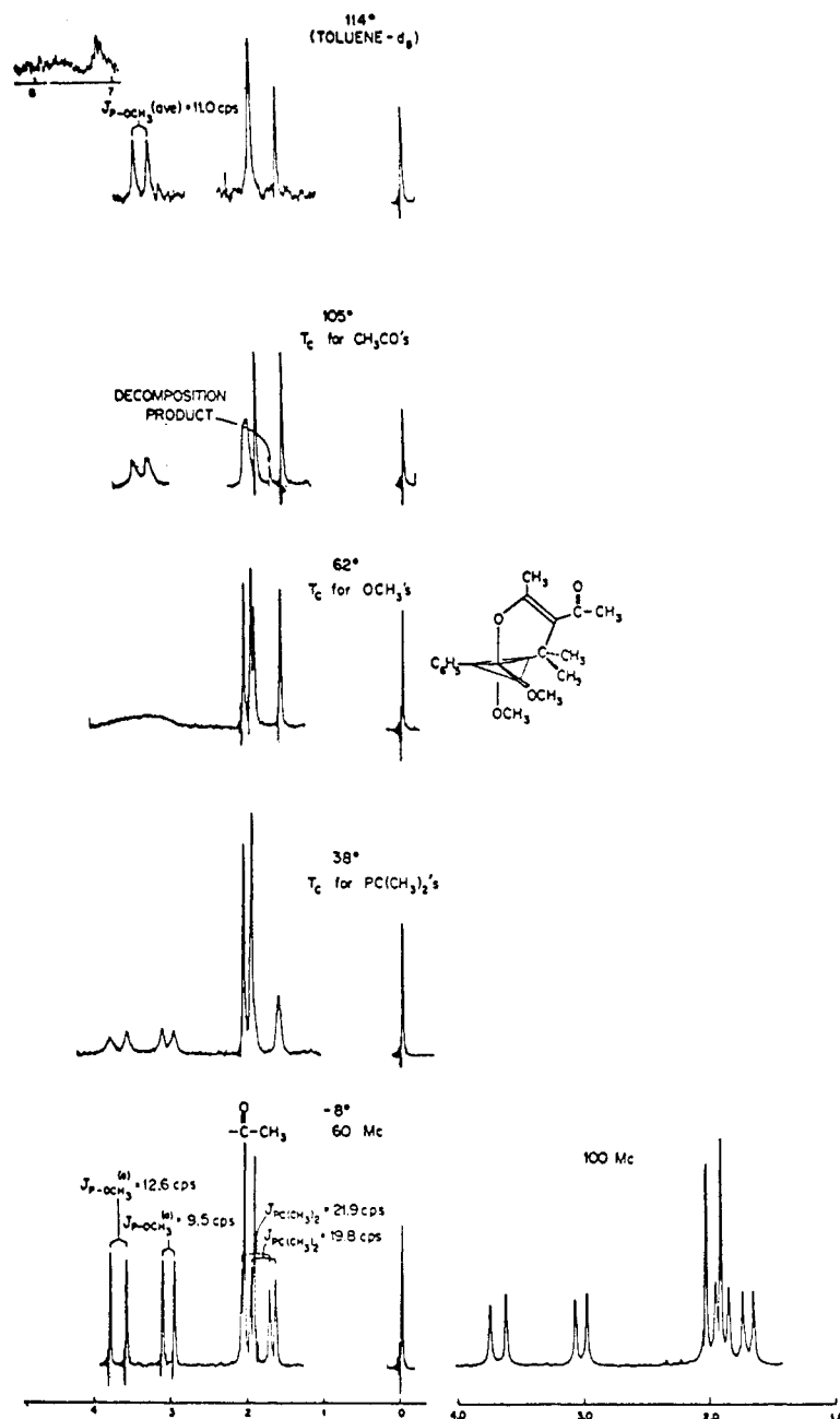
Figure 2. Temperature dependence of the nmr spectrum of the adduct 4 of dimethyl phenylphosphonite and isopropylideneacetylacetone (60 Mc except where otherwise indicated; bromobenzene as solvent except where otherwise indicated).
