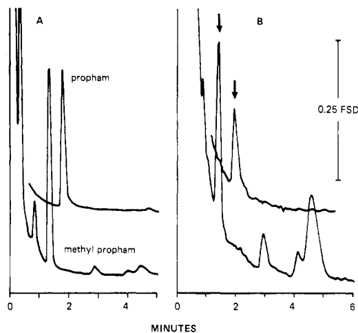
Figure 4. Gas chromatograms of propam and alkylated propam (2- and 0.48- \mu g levels): (A) 24 ng of propam, before and after alkylation (2 \mu g); (B) 24 ng of propam, before and after alkylation (0.48 \mu g).
