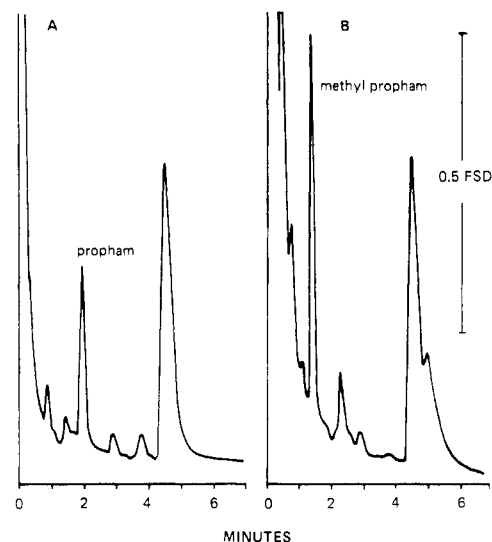
Figure 5. Gas chromatograms of crude chloroform extract of potatoes fortified with propam (0.5 ppm), before and after alkylation: (A) crude potato extract; (B) alkylated potato extract.
