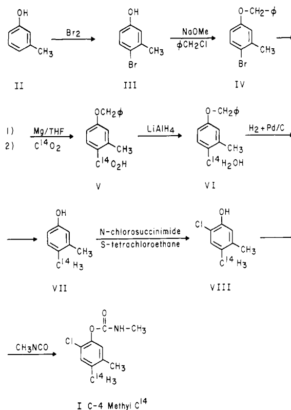
Figure 1. Synthesis of 2-chloro-4,5-dimethylphenyl N -methylcarbamate 4-methyl C^{14}
