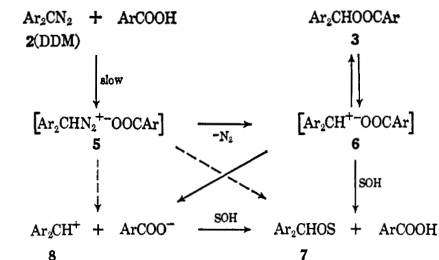
Chart II. Ar \equiv C 6 H 5
