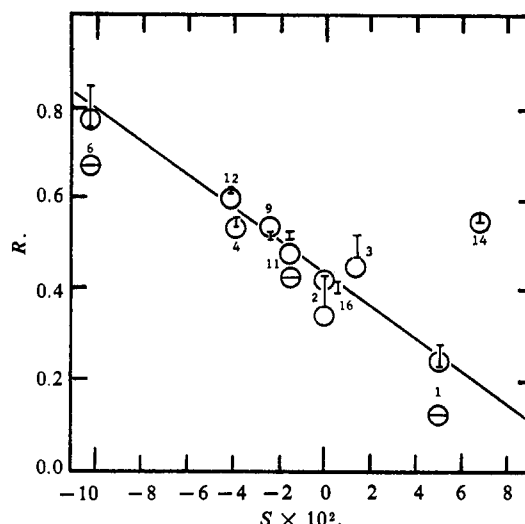
Figure 2. The effect of the solvent polarity on product partitioning, R , in the decomposition of N-nitroso-N-benzhydrylbenzamide in hydroxylic solvents (solvent polarity parameter, S , from ref 24; R values and solvents are given in Table I). Vertical bars, data of E. R. S.; circles, data of J. G.; circles with horizontal bars derive from the 37% sample (see Table I, footnote m ).
