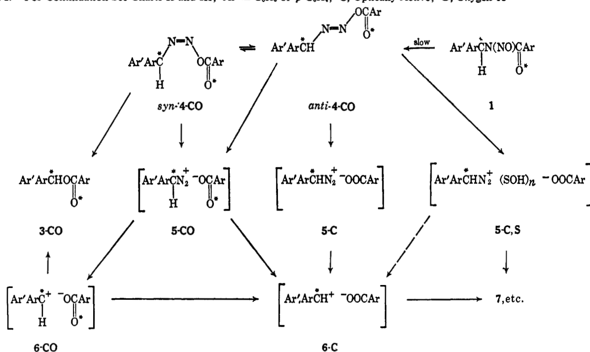
Chart II. Ar \equiv C 6 H 5
