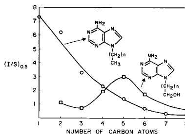
Fig. 1—A plot of the index of inhibition vs. the number of carbons in the 9-substituent of some 9-(alkyl)- and 9-(hydroxyalkyl)adenines.
