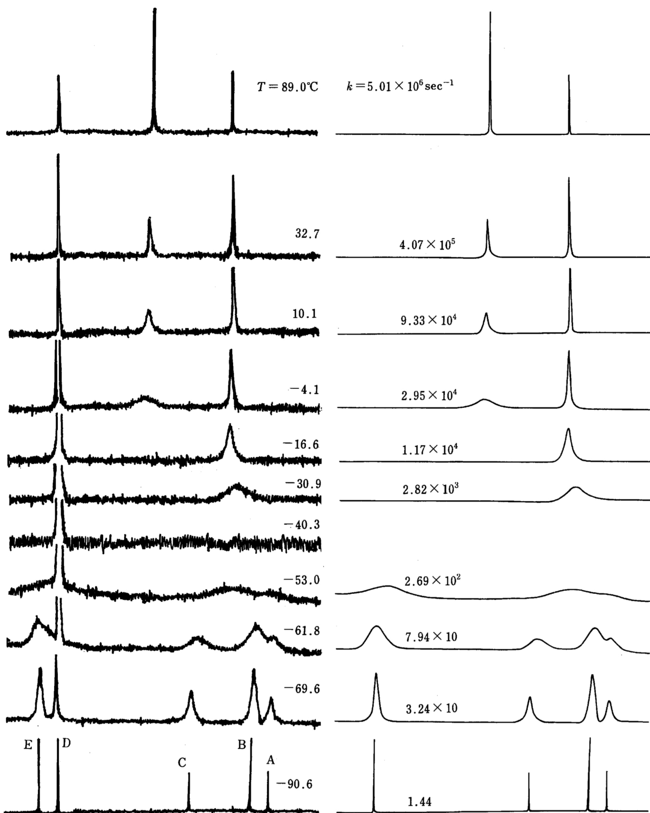
Fig.1. The observed (left) and the calculated (right) spectra of methine carbons of barbaralone at several temperatures. (The peaks of nonexchanging carbons, D, are not included in the calculated spectra.)
