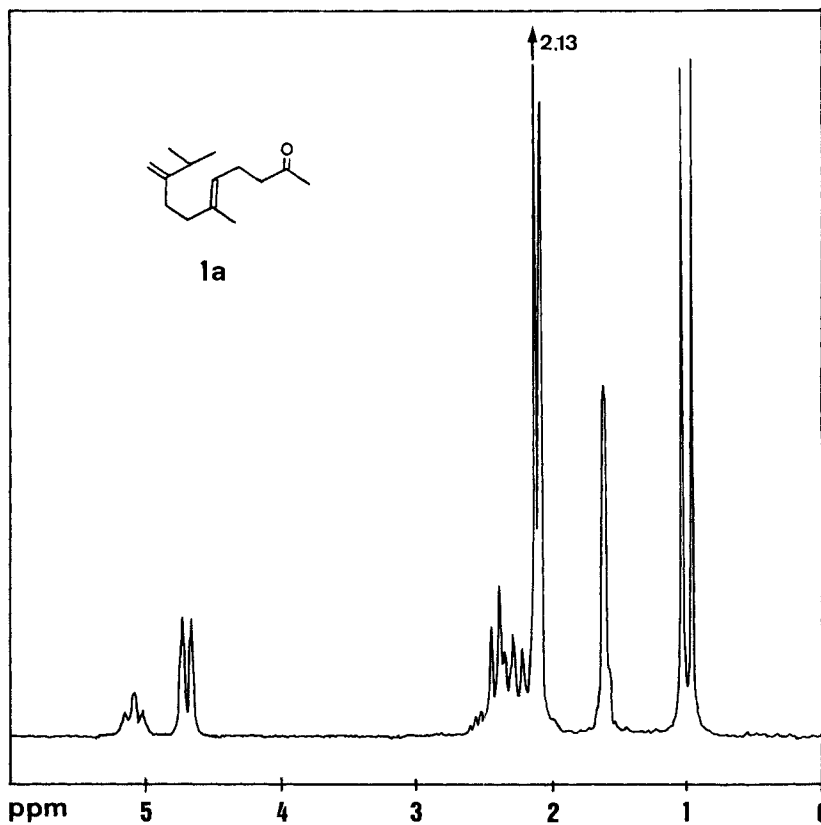
Fig. IR. (liquid film) and NMR. (90 MHz, \text{CDCl}_3 ) spectra of (E)-9-isopropyl-6-methyl-5,9-decadien-2-one ( 1a )
