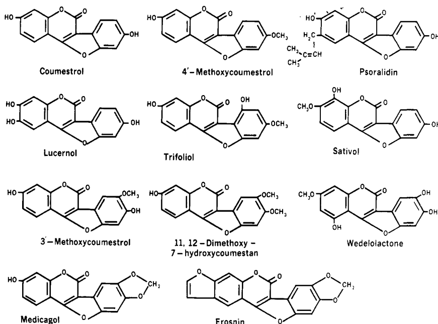
Figure 1. Naturally occurring coumestans
