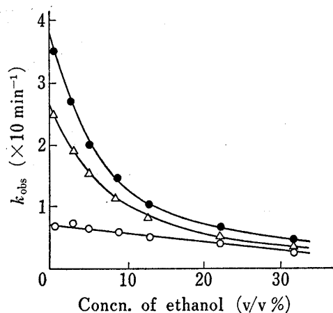
Fig. 6. Effect of Ethanol Concentration on Rate of Isomerization of \text{PGA}_1 in the Absence and in the Presence of CyDs ( 5 \times 10^{-3} \text{ M} ) in Phosphate Buffer (pH 11.4, \mu=0.2 ) at 60^\circ
