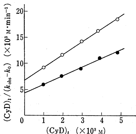
Fig. 2. Determination of K_e and k_e for \text{PGA}_1 -CyD Complexes from Kinetic Data (Fig. 1) according to Eq. (1)
