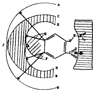
Fig. 1.—Scale model cross section of a possible relationship of the active site to the enzymic nucleophilic site. The horizontal cross-hatch represents the part of the enzyme with the active-site. See Discussion for the significance of the vertical and angular cross-hatch. The short arrow represents the most extended conformation of the -\text{CH}_2\text{CONH}- group and is 3.7Å. long from the center of the methylene carbon to the N -phenyl bond; the long arrow represents the -\text{CH}_2\text{CONHCH}_2- group which is 7.7Å. long when fully extended. The measurements were made with Leybold models.
