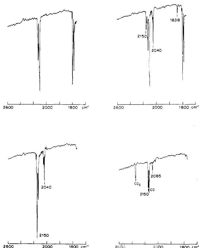
Figure 1. Infrared spectra of 1 matrix isolated in argon at 8 K before irradiation (upper left), after irradiation ( >274 nm) for 1 min (upper right), after irradiation ( >274 nm) for 10 min (lower left), and after irradiation with quartz optics for 524 min (lower right). Note the scale change at 2000\text{ cm}^{-1} .
