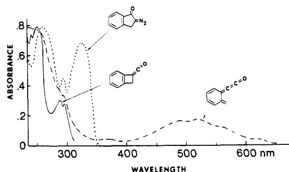
Figure 3. Dotted line, 10 in 2-MeTHF; dashed line, 9 (with some 8 ) generated by photodecomposition of 10 with ultraviolet light (254 nm); solid line, 8 after bleaching of 9 away with visible light. All spectra and photochemistry at 77 K.
