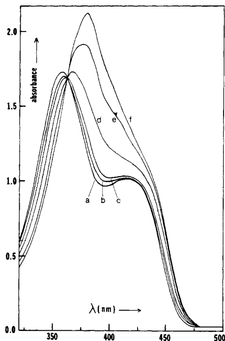
Figure 1. Optical spectra of a 10^{-3} M THF solution of potassium picrate in the presence of varying amounts of 4'-carbomethoxybenzo-15-crown-5 (compound I) at 25^{\circ} . Molar ratio of crown ether to picrate salt: (a) 0; (b) 1.00; (c) 1.85; (d) 6.83; (e) 24.9; (f) 180.
