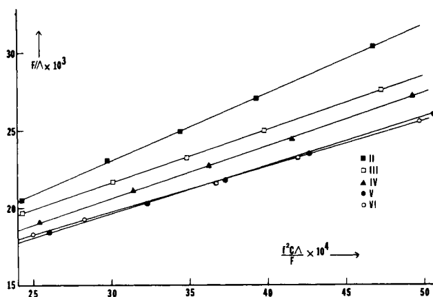
Figure 3. Plots of F/\Delta vs. f^2c\Delta/F in THF at 25° for complexes of potassium picrate with the macrobicyclic polyethers II (■), III (□), IV (▲), V (●), and VI (○).
