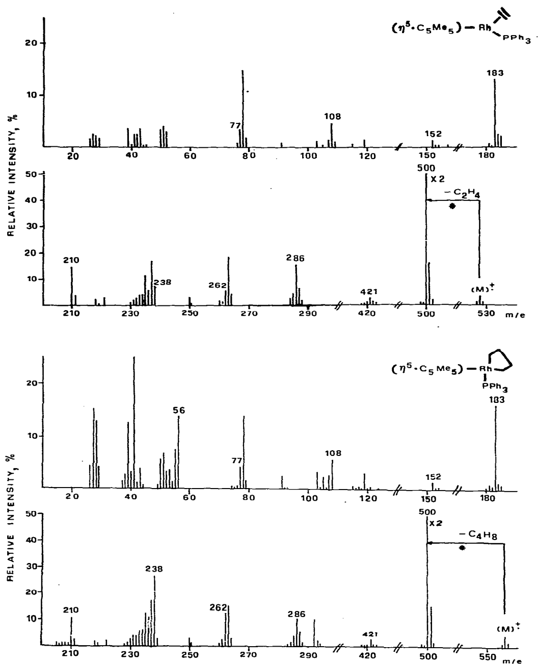
Fig. 1. Mass spectra of (triphenylphosphine)(ethylene)(pentamethylcyclopentadienyl)rhodium (III) (top), and of (triphenylphosphine)(butane-1,4-diyl)(pentamethylcyclopentadienyl)rhodium (IV) (bottom).
