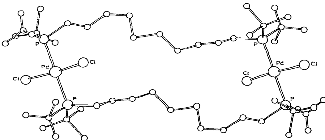
Fig. 3. The structure of trans -[PdCl 2 { t -Bu 2 P(CH 2 ) 10 P- t -Bu 2 }] 2 showing the 26-atom ring.
