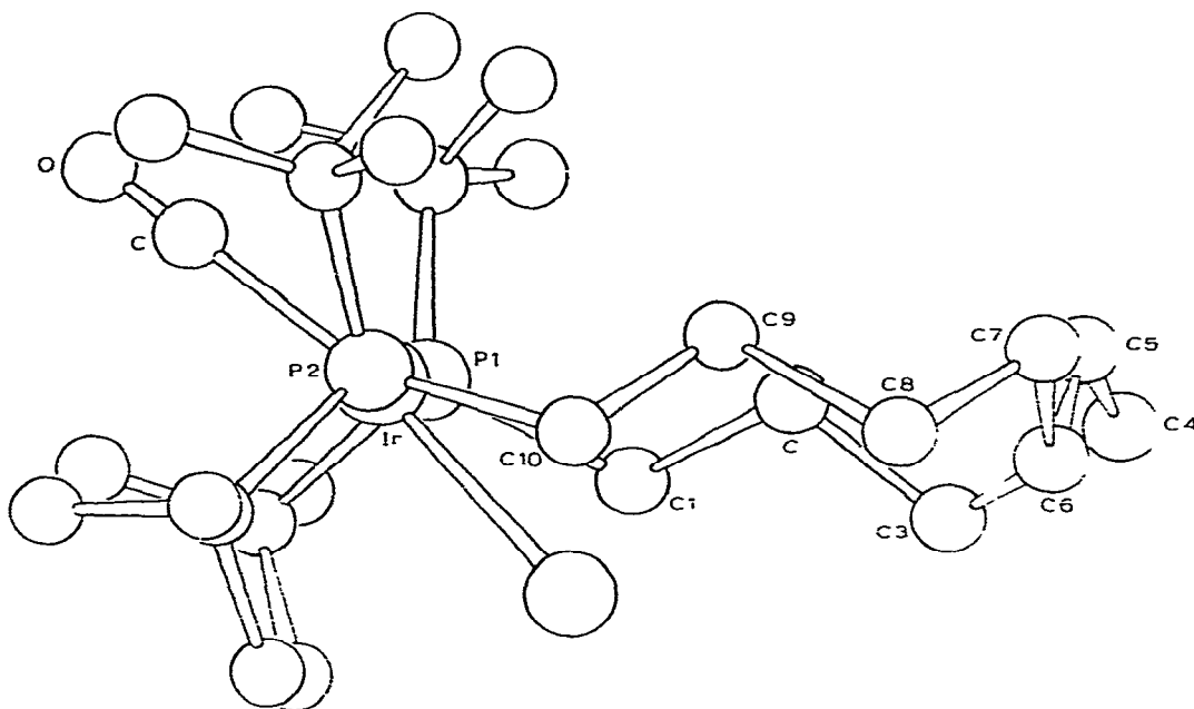
Fig. 2. trans -[IrCl(CO){ t -Bu 2 P(CH 2 ) 10 P- t -Bu 2 }]. View along the P—Ir—P bonding.
