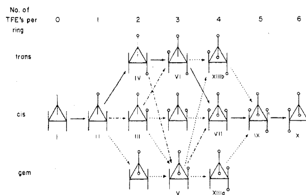
Figure 2. Possible reaction pathways for the replacement of chlorine in (\text{NPCl}_2)_3 by trifluoroethoxy groups. The circles represent trifluoroethoxy groups, and the solid arrows depict the principal pathway found in this work. The lines made up of dots and dashes represent the formation of the minor products. "TFE's per ring" refers to the number of trifluoroethoxy groups.
