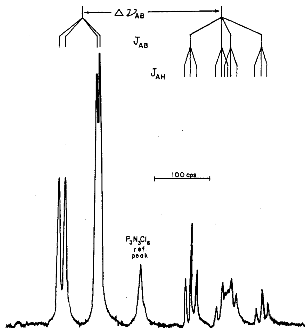
Figure 1. ^{31}\text{P} NMR spectrum of \text{N}_3\text{P}_3\text{Cl}_5(\text{OCH}_2\text{CF}_3) measured at 40.5 MHz. The spectrum can be interpreted as an \text{AB}_2\text{X}_2 pattern.
