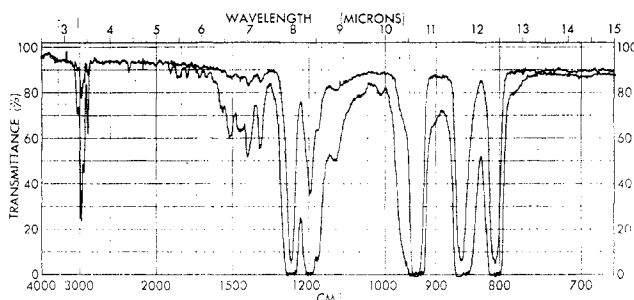
Figure 3.—Infrared absorption spectra of (\text{CH}_3\text{NPF}_3)_2 .
