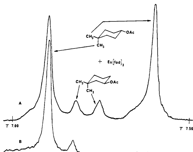
Figure 1. Geminate dimethyl pmr spectra at 100 MHz: (A) 4,4-dimethylcyclohexyl (87%) and 3,3-dimethylcyclohexyl (13%) acetates 2.6 M in carbon tetrachloride plus 0.10 M \text{Eu}(\text{fod})_3 ; (B) acetates 4 and 5 from solvolysis of labeled tosylate 1, same sample conditions.
