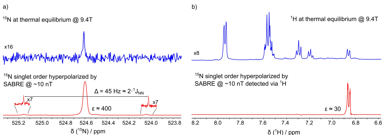
Figure 7. ^{15}\text{N} NMR spectra (a) and ^1\text{H} NMR spectra (b) showing a comparison of ^{15}\text{N}_2 -ABZ signals in thermal equilibrium (blue) and after SABRE SHEATH hyperpolarization at 10 nT of the singlet order of the ^{15}\text{N} spin pair (red). The thermal spectrum in (a) was acquired in 4 scans with proton decoupling. This narrowed the line and increased SNR. Hyperpolarized ^{15}\text{N} spectrum exhibits outer singlet-triplet coherences. The experimental protocol for the SABRE experiments is shown in Figure 2b.
