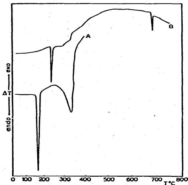
Fig. 1. A = Dibenzo-18-crown-6 (1); B = complex of (1) and potassium iodide.
