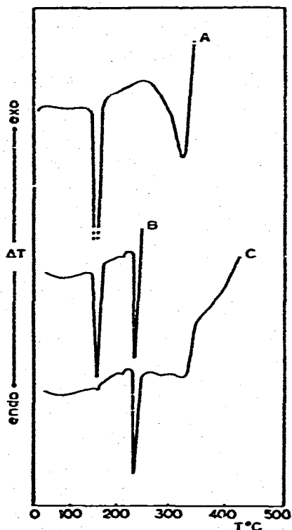
Fig. 2. A = Dibenzo-18-crown-6 (1); B = mixture of KI and (1); C = reheating of B.
