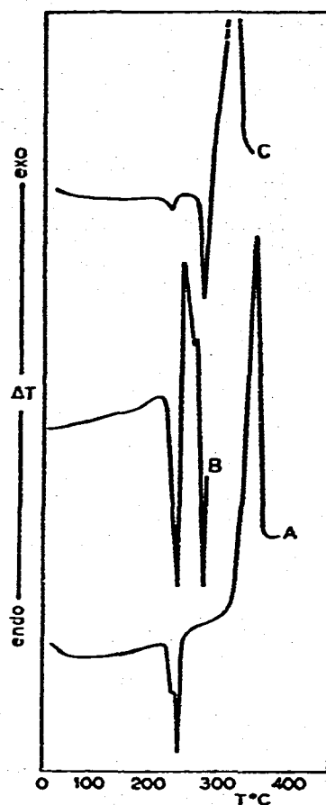
Fig. 2. A = Dibenzo-18-crown-6 (1); B = mixture of KI and (1); C = reheating of B.
