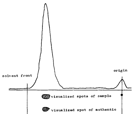
FIG. 2. Radio-thin-layer chromatogram of gefarnate- ^{14}\text{C}
