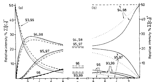
Figure 2. Effect of the competition factor \beta = ([Z]^+ \rightarrow [1]^+)/([Z]^+ \rightarrow [1]^+) + [Z]^+ \rightarrow [2]^+) on the variation of the [C_7(H, D)_8]^+ abundance patterns with the number n of exchange cycles, calculated for (a) 1f and (b) 1g . — \beta = 0 , ---- \beta = 1 .
