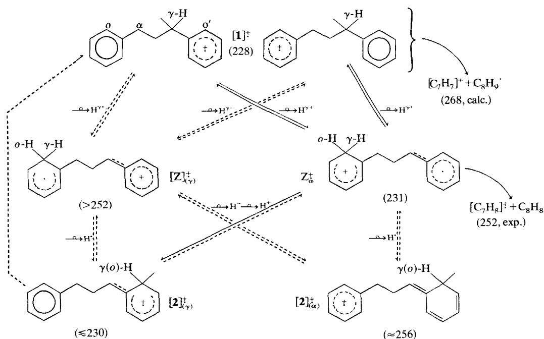
Scheme 5. Isomerization occurring in the molecular ions of 1 before fragmentation to [C_7H_7]^+ and [C_7H_8]^+ . Values refer to the corresponding enthalpies of formation in kcal mol -1 . Full arrows represent main reaction paths (see text).
