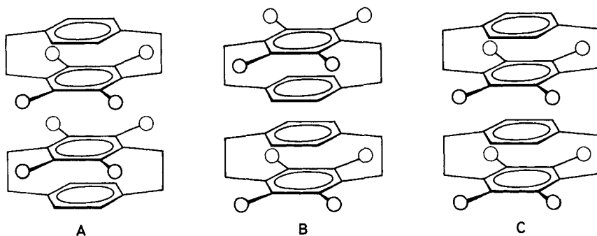
Fig. 4. The three alternative structures for the dimeric radical cation I_2 \cdot^+ in which the two molecules of 4,5,7,8-tetramethyl[2.2]paracyclophane (I) lie in parallel planes and in an essentially eclipsed arrangement. The circles represent methyl groups.
