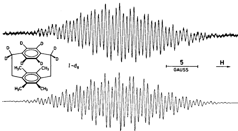
Fig. 2. ESR. spectrum of the dimeric radical cation (I-d_8)_2 \cdot^{\oplus} . Top: experimental spectrum taken under the same conditions as that in Figure 1. Bottom: computer simulated spectrum. Coupling constants (Gauss): 2.23 (24H), 1.68 (8H), 0.054 (8D) and 0.028 (8D). Line-shape: Lorentzian; line-width: 0.16 Gauss.
