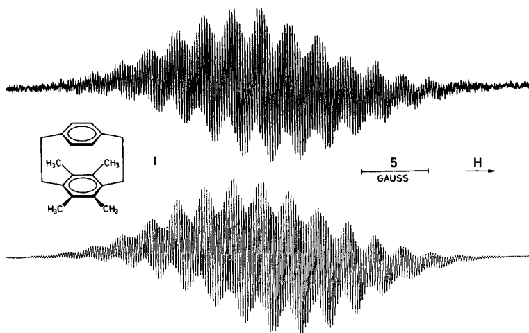
Fig. 1. ESR. spectrum of the dimeric radical cation I_2 \cdot^{\oplus} . Top: experimental spectrum. Solvent: \text{CH}_2\text{Cl}_2/\text{CF}_3\text{COOH}/(\text{CF}_3\text{CO})_2\text{O} 10:1:1; Temp.: -80^\circ . Bottom: computer simulated spectrum. Coupling constants (Gauss): 2.23 (24H), 1.68 (8H), 0.35 (8H) and 0.18 (8H). Line-shape: Lorentzian; line-width: 0.16 Gauss.
