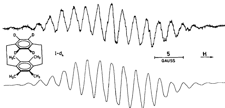
Fig. 3. ESR. spectrum of the dimeric radical cation (I-d_4)_2 \cdot^+ . Top: experimental spectrum taken under the same conditions as that in Figure 1. Bottom: computer-simulated spectrum. Coupling constants (Gauss): 2.23 (24H), 1.68 (8H), 0.18 (8H) and 0.054 (8D). Line-shape: Lorentzian; line-width: 0.20 Gauss.
