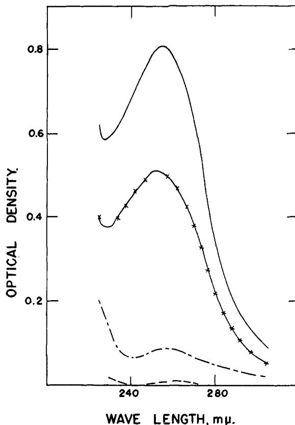
Fig. 2.—Curve A, fresh solution of 2-nitriminoimidazolidine in N KOH, —; curve B, same solution after 4 hours, ×—×; curve C, solution after 24 hours, - - -; curve D, solution after 48 hours, — · —.
