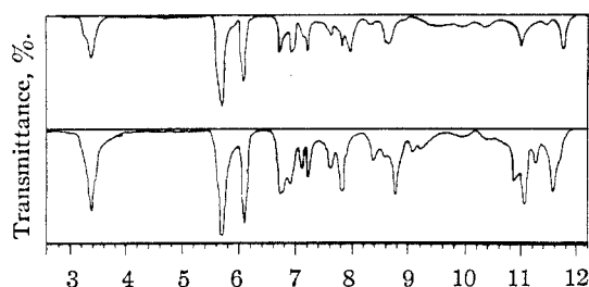
Fig. 1.—Infrared absorption spectra: top curve, umbellulone dibromide (II) in carbon tetrachloride; bottom curve, bromodihydroumbellulone (III) in carbon tetrachloride.
