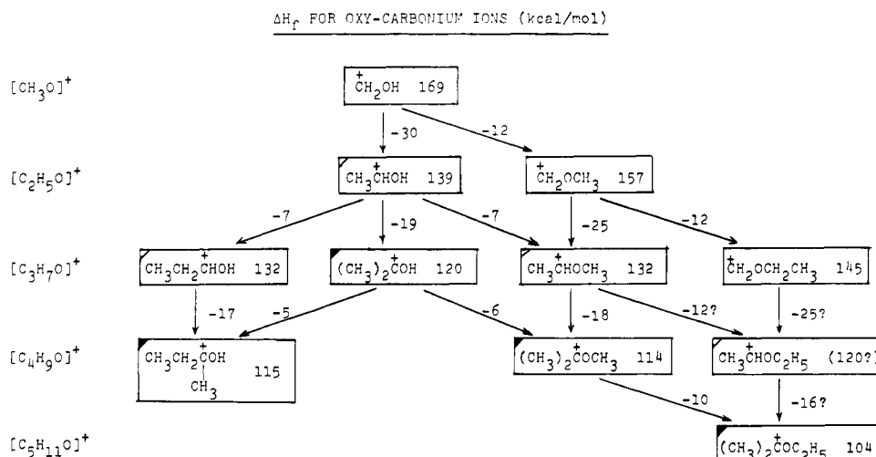
Figure 2. Schematic illustration of the relationships in heats of formation of oxycarbonium ions (ΔH f (ion) in kcal/mol). Secondary and tertiary ions are identified by corner markings. Vertical arrows correspond to CH 3 substitution on charged atoms, slant arrows correspond to CH 3 substitution on uncharged atoms.
