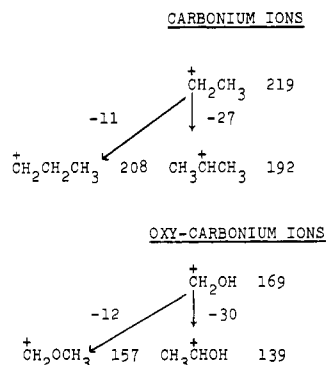
Figure 1. The stabilizing effect of substituting CH 3 for H in carbonium and oxycarbonium ions. Note that the effect of substituting CH 3 for the hydroxyl H in CH 2 OH ion is similar to that for substitution on the "uncharged" atom in the + CH 2 CH 3 ion. Substitution on the C atom in + CH 2 OH ion has a much greater stabilizing effect, comparable to substitution on the "charged" C atom in + CH 2 CH 3 ion. Numbers are ΔH f (ion) in kcal/mol.
