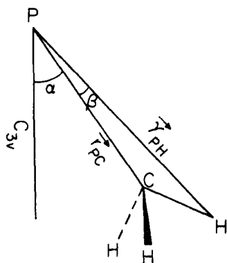
Figure 1. Analysis of the dipolar coupling in a nonrigid pyramidal \text{YP}(\text{CH}_3)_3 molecule. \gamma_{\text{PC}} and \gamma_{\text{PH}} refer to internuclear distance vectors.
