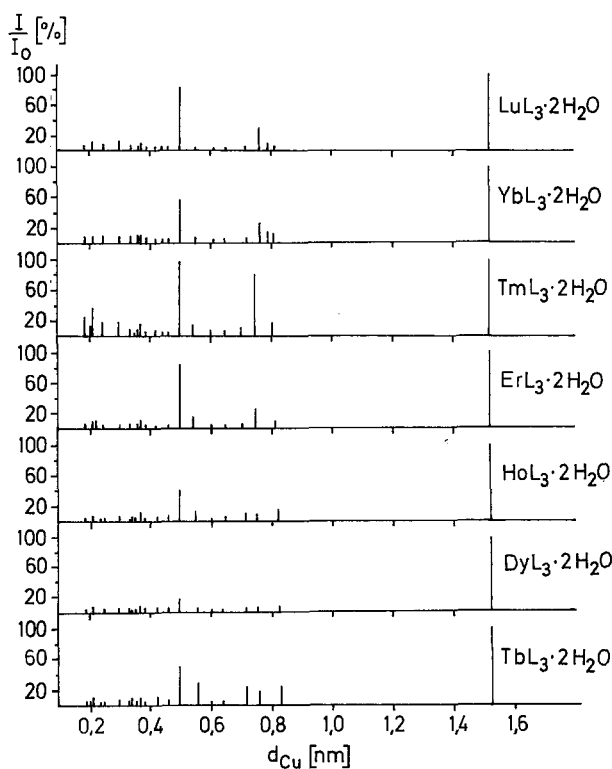
Fig. 2. Powder photograph of anthranilates \text{Ln}(\text{C}_6\text{H}_4\text{NH}_2\text{COO})_3 \cdot 2\text{H}_2\text{O} where \text{Ln} = \text{Tb} - \text{Lu}
