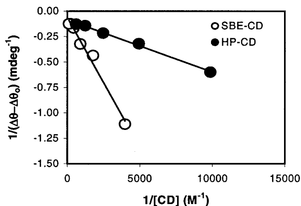
Fig. 4. 1/\Delta\theta vs. 1/[CD] , where \Delta\theta is the ellipticity difference between the bound and free species of the ring opened form of DB-67 ( II^{2-} ) and [CD] is the cyclodextrin concentration. The lines are least-squares fits using Eq. (5).
